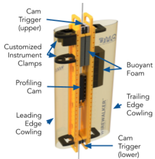
Figure 4: Illustration of the basic anatomy of a Wirewalker Profiler
