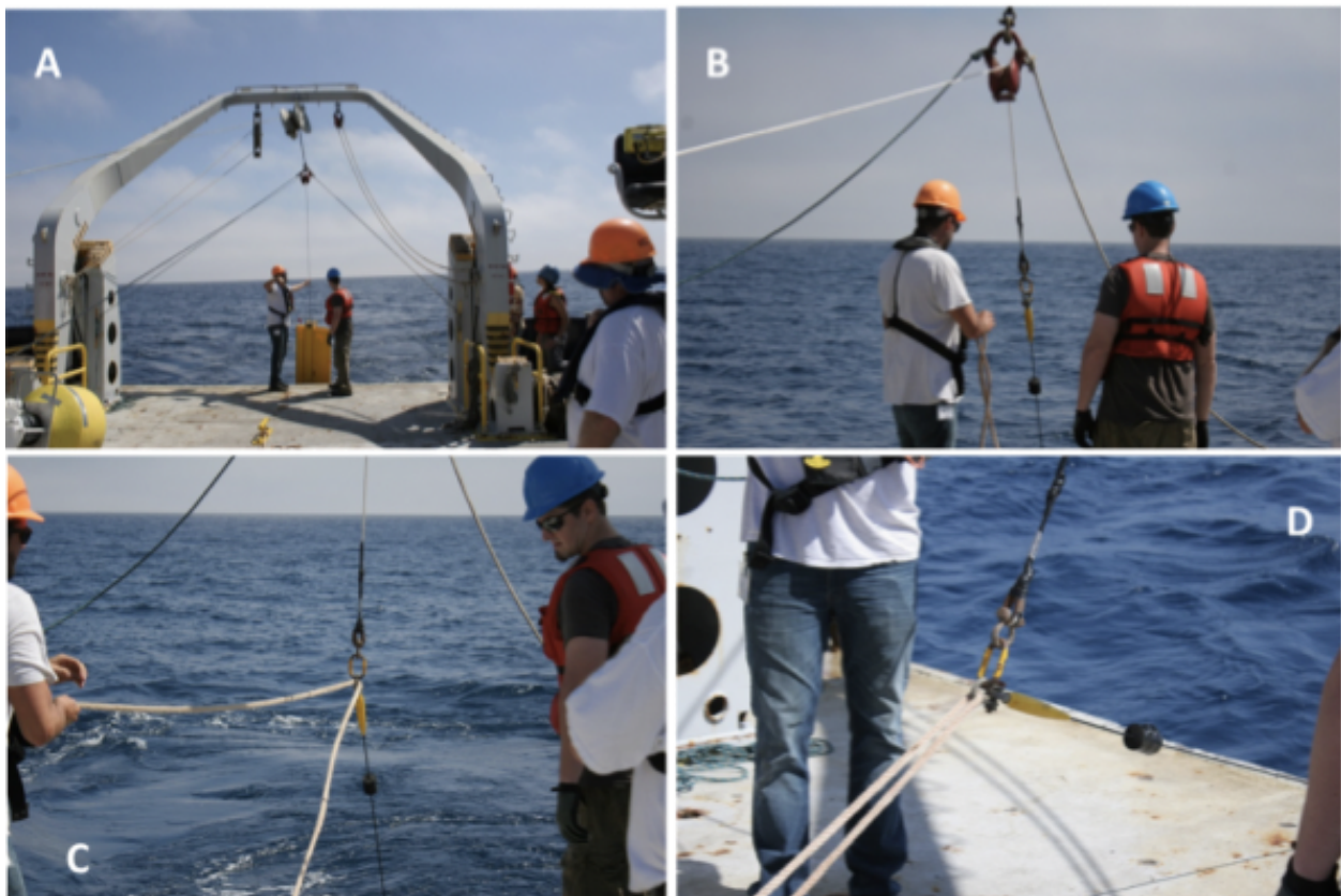
Figure 11: Deployment of the Wirewalker - (A) Lowering the Wirewalker into the water; (B) through (D) Stopping the line off to the deck to connect the surface buoy.
