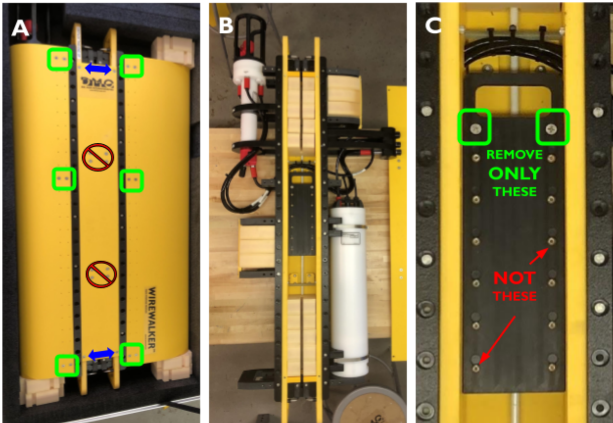
Figure 5: The cowlings, center lid, and cam can all be opened using a common #3 Phillips Screwdriver. Other types of hardware (hex drive) need NOT be removed. A) A WW with cowling and center lid installed. Green Squares identify the cowling screws and Blue Arrows are used to identify the central lid screws. B) With lid removed, the cam is visible (black box in center). C) Close up of the cam box. Green Squares identify the large Phillips screws used to open the cam. The smaller hex head screws in the keyholes should NOT be adjusted.
