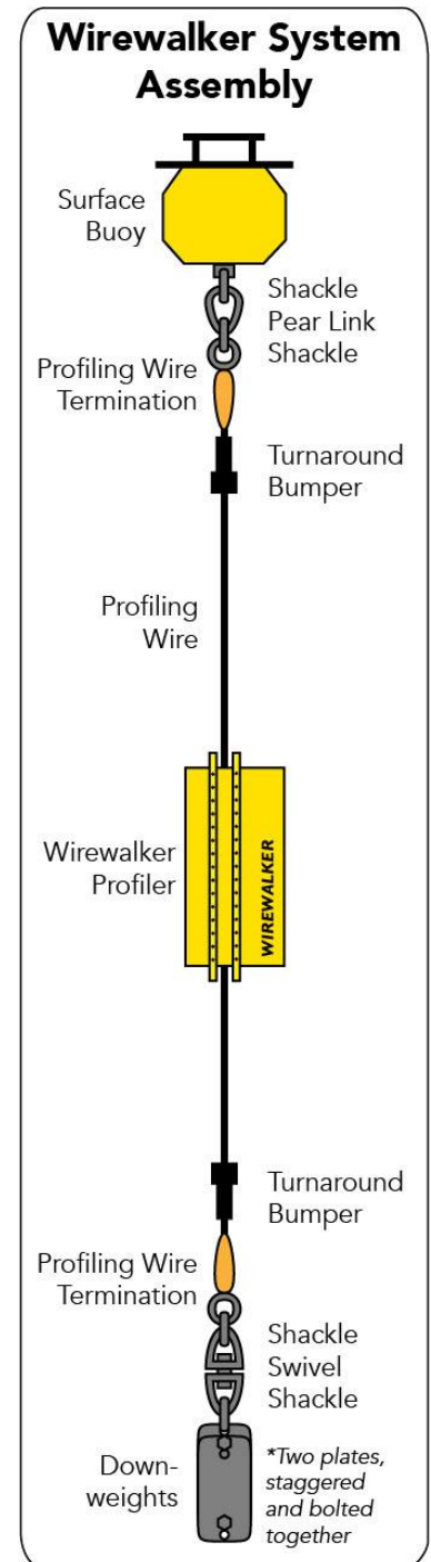
Figure 3: Wirewalker Profiling System Components and Assembly. As-is the system is ready for free-drifting deployments. Additional hardware and mooring tackle is required for moored deployments.
