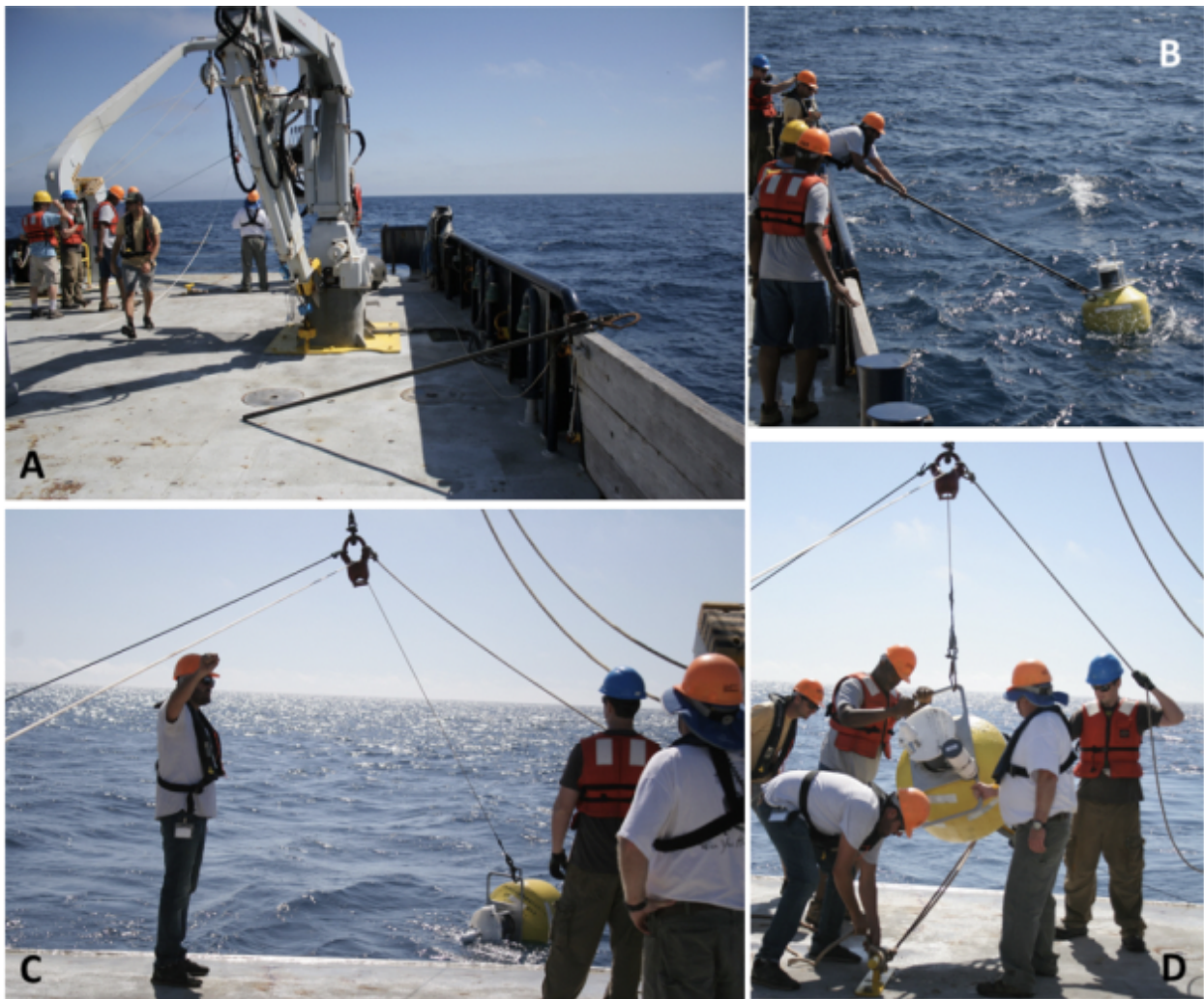
Figure 13: Retrieval Process - (A) Boat hook with capture hook. A line is run from the winch around the stern and connected to the capture hook; (B) Capturing the Wirewalker with the hook as it drifts by; (C) Winching the Wirewalker in; (D) Stopping the surface.
