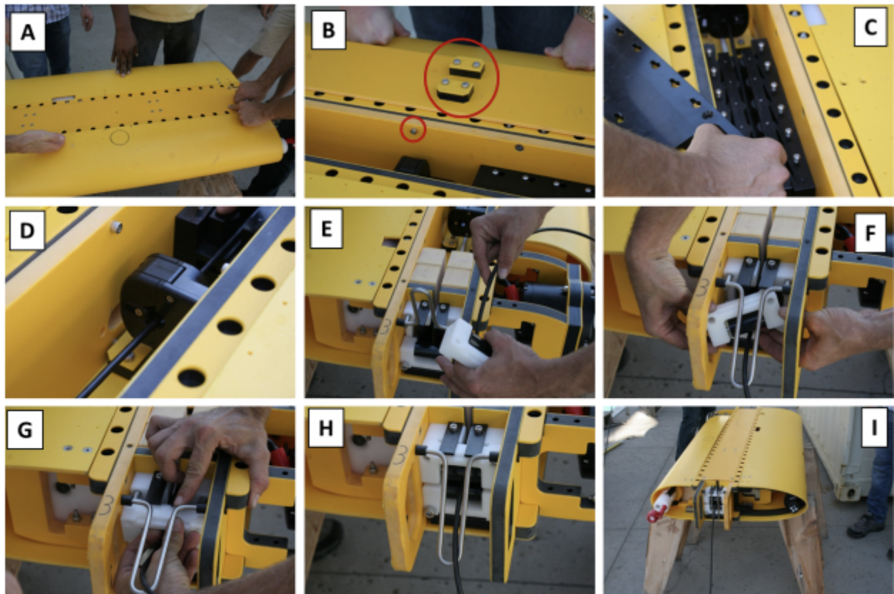
Figure 6: Step-by-step connection of the vertical profiler to the jacketed profiling wire.
