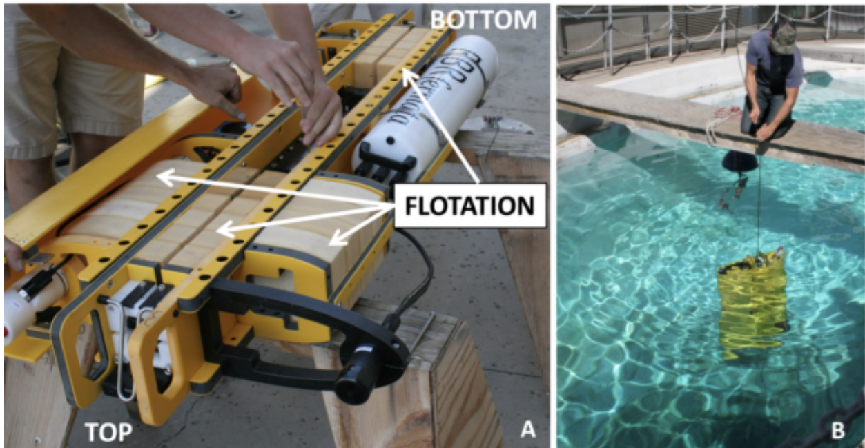
Figure 8: (A) Location of Wirewalker buoyancy foam; (B) Hands-on ballasting of the Wirewalker at Scripps Institution of Oceanography using their 10 m test tank.
