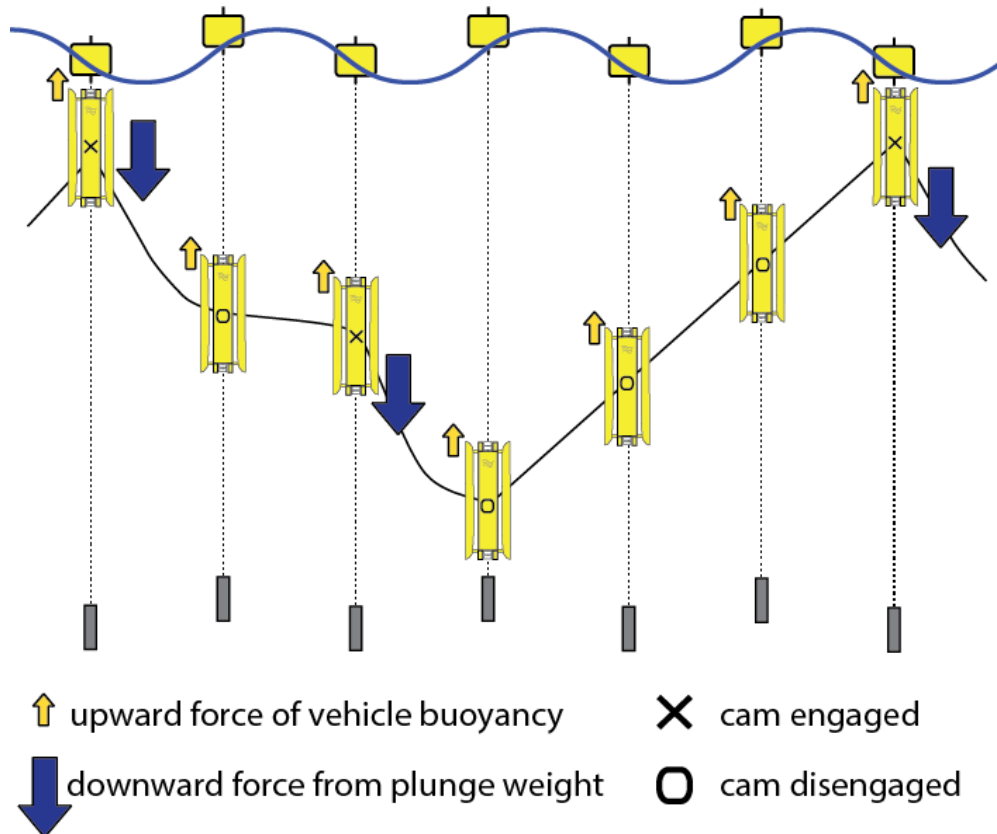
Figure 2: Profiling cycle of the Wirewalker.
